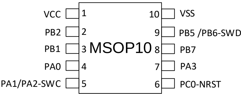
图 3-1 MSOP10 Pinout1 PY32M010A15N6
